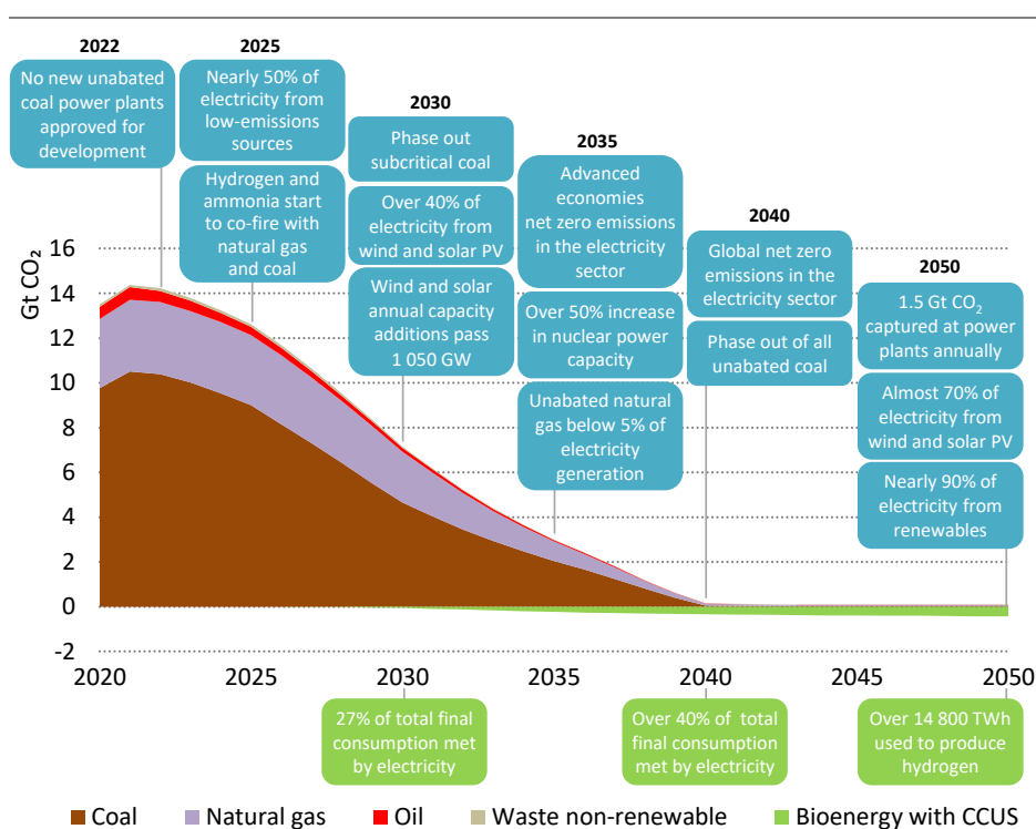
Figure 3.9 ▶ CO 2 emissions by source and key milestones in the electricity sector in the NZE Scenario, 2020 to 2050
