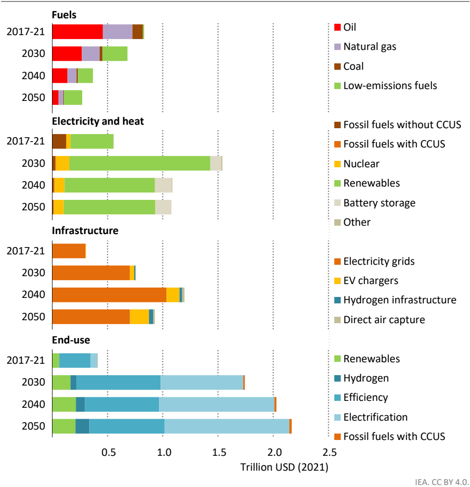
Figure 3.22 ▶ Global average annual energy investment by sector and technology in the NZE Scenario
