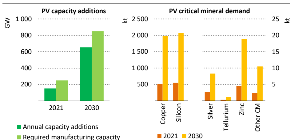
Figure 3.27 ▶ Solar PV capacity additions and mineral demand in the NZE Scenario, 2021 and 2030
