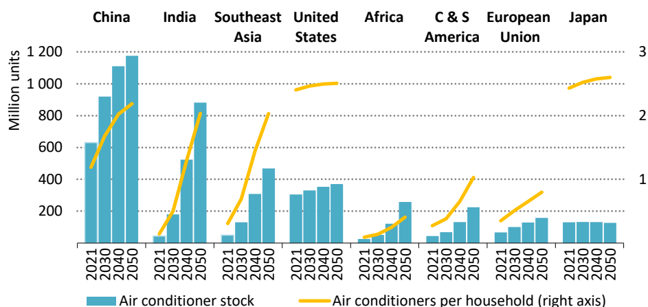
Figure 5.19 ▶ Household air conditioner ownership in selected regions in the STEPS, 2021-2050
