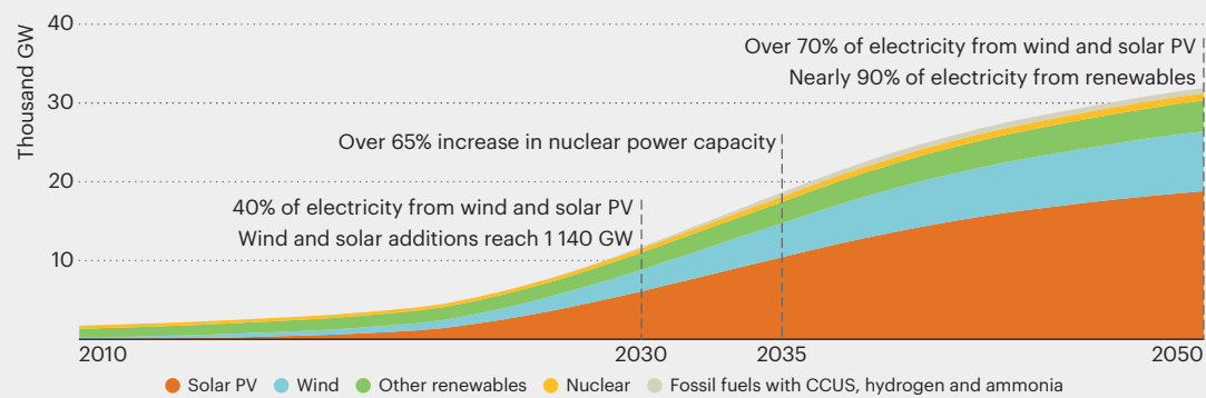
Low-emissions electricity generation capacity by source
